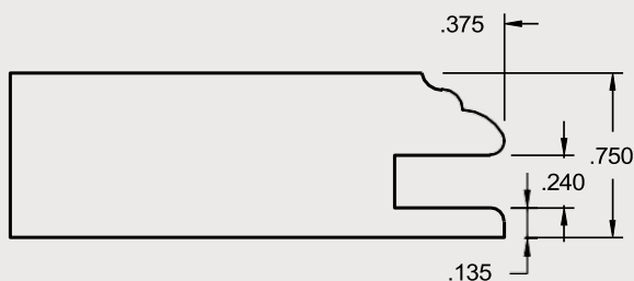
TWIN BEAD
